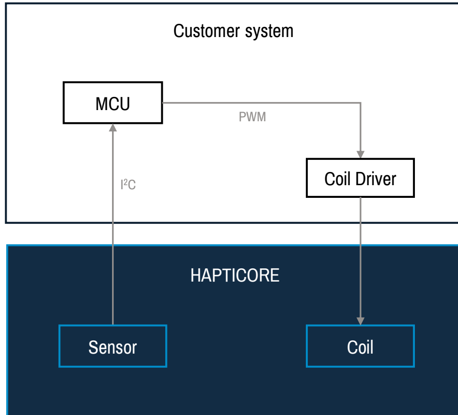
Option 1: HAPTICORE to customer system
