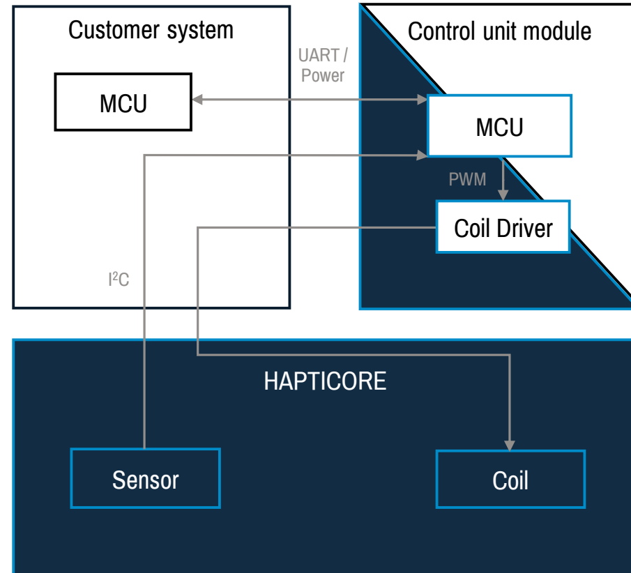
Option 2: HAPTICORE to control unit module
